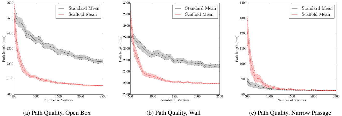
Figure 2: Path quality over the number of vertices in the base graph for the fixed configurations
